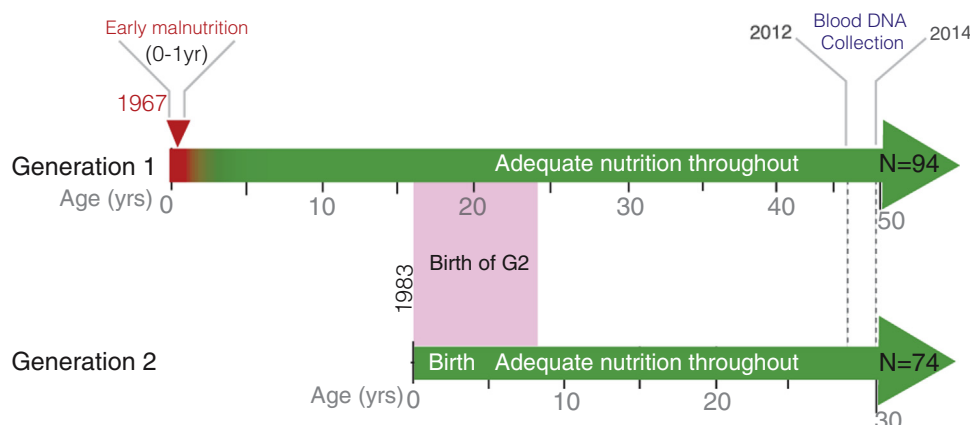
Figure 1. Overview and timeline of the Barbados Nutrition Study. Generation 1 ( n = 94 ) included 44 control subjects and 50 subjects who were malnourished during the first year of life. Subjects with a history of early life malnutrition enrolled in a government-sponsored intervention program that included nutrition education, food subsidies, routine health care, home visits, and a preschool program that extended to 12 years of age. Approximately 44 years after exposure to malnutrition, blood was drawn by venipuncture for the DNA methylation scan. Generation 2 ( G2 ; n = 74 ), all offspring of members of generation 1 (44 offspring of generation 1 subjects with early mal-
