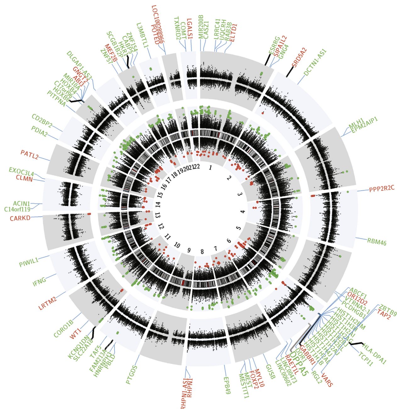
Figure 3. Genome-wide DNA methylation changes in previously malnourished generation 1 subjects and their generation 2 offspring. Circos plot depicting the entire autosomal complement, green (red) genes with transcription start sites within \pm 2 kb of significantly hyper-(hypo-)methylated differentially methylated genomic regions. Genes with thin connector (gene abbreviation to plot) line = generation 1; thick connector = generation 2. The black innermost ring (with vertical lines) represents autosome ideograms (annotated is the chromosomal number), with the pter-qter orientation in a clockwise direction. The dots on the inner side (negative) and outer side (positive) of the ideogram represent Fisher's -\log_{10}(p) value for each 1-kb window analyzed in generation 1. Each dot marks the location of the Illumina 450K probe along the genome. The next outermost black circle (with dots on the inner/negative and outer/positive side) represents Fisher's -\log_{10}(p) value for each 1-kb window analyzed in generation 2. DPPA5 (green, larger font) was significantly hypermethylated in both generation 1 and generation 2 cohorts. Only genes where the differentially methylated genomic region overlaps its promoter (i.e. \pm 2 kb of transcription start site [TSS]) are shown.
