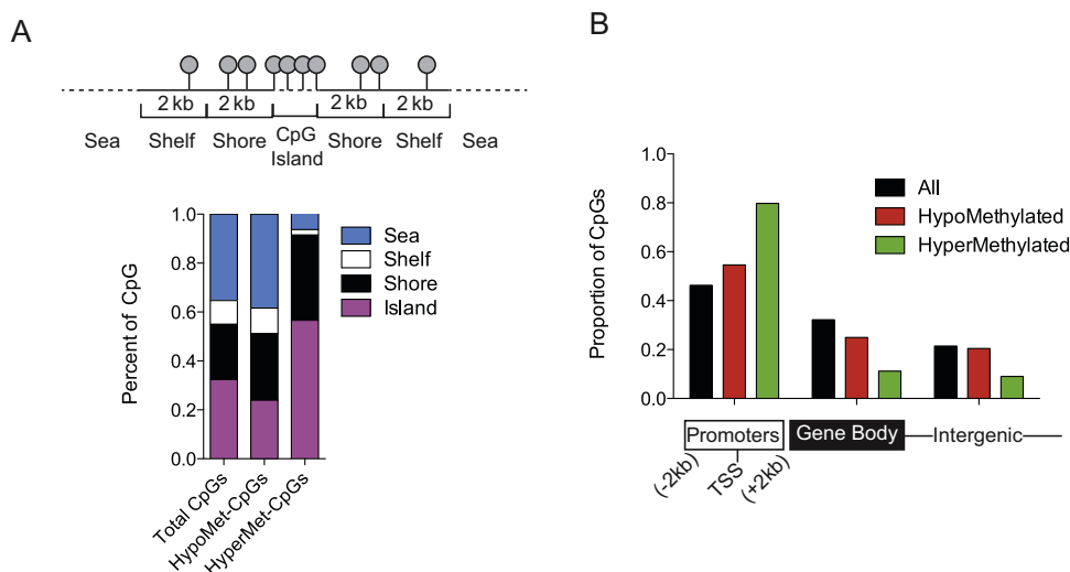
Figure 2. Genome-wide distribution of DNA methylation changes after malnutrition. Distribution of CpG sites (A) in CpG islands, shores, shelves, and sea and (B) relative to RefSeq gene promoters, gene bodies, and intergenic regions. CpGs in hypomethylated and hypermethylated differentially methylated genomic regions are compared with all autosomal CpGs (total CpGs) on the Illumina array using Pearson's \chi^2 test. Note pronounced (approximately two-fold) overrepresentation of hypermethylated differentially methylated genomic regions at CpG islands and gene promoters.
